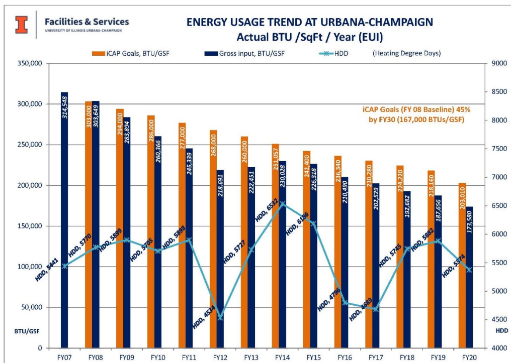
Figure 2. Energy usage trend for Actual BTU/Sq.Ft./Year (EUI).
