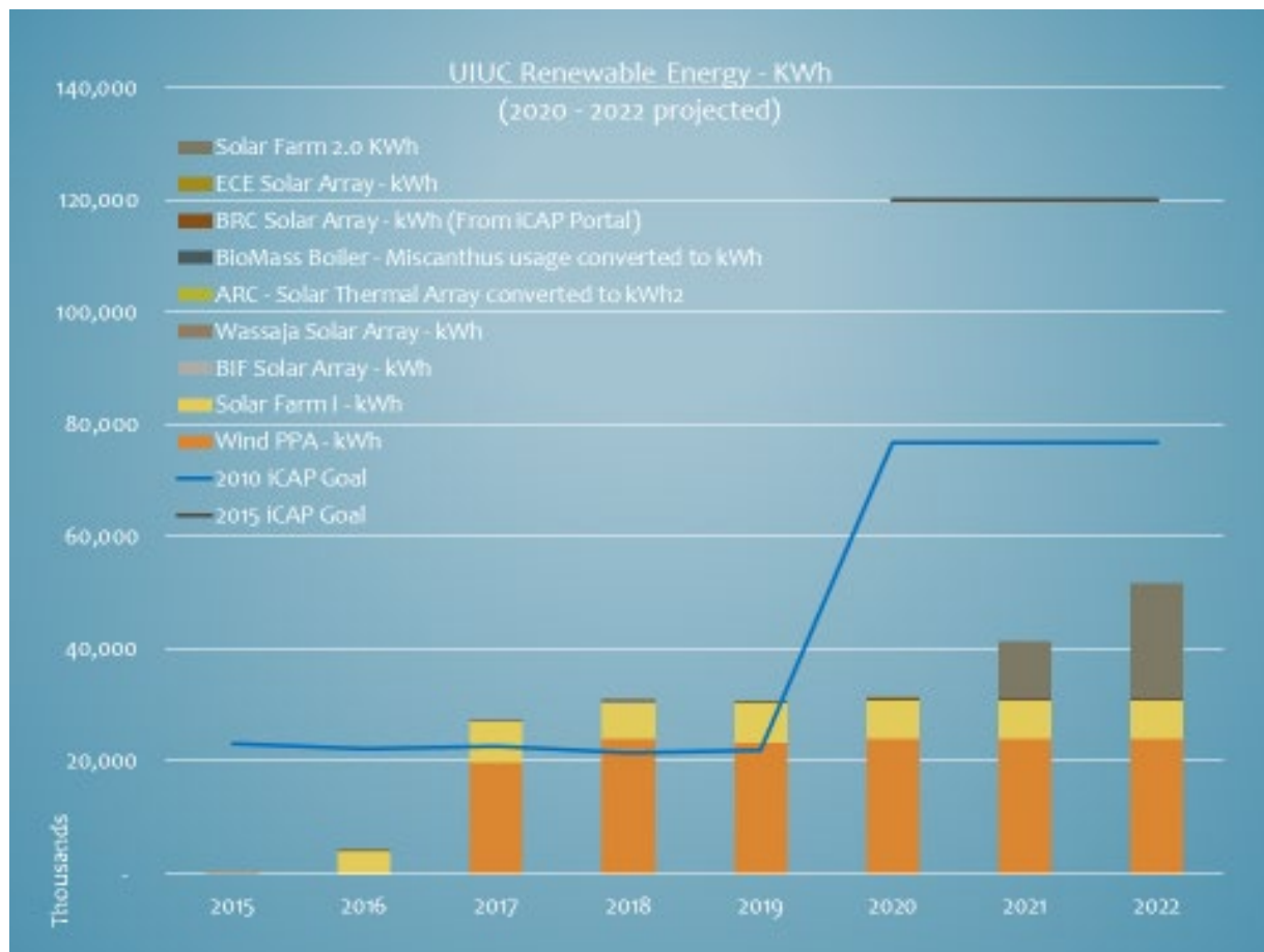
Figure 10. UIUC renewable energy - kWh.
